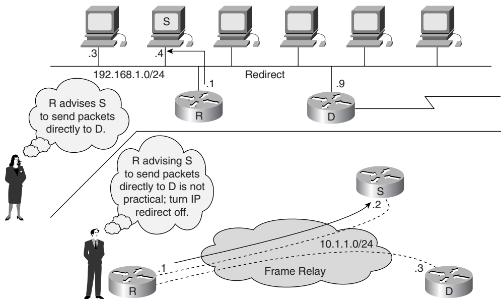
Figure 10-1 IP Redirects
